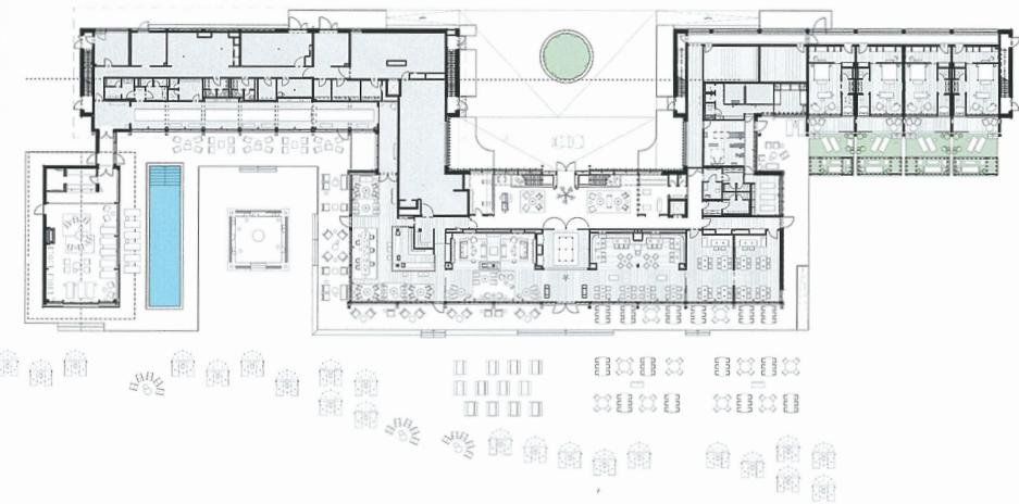
Grundriss Edgeschoss • Ground floor plan
